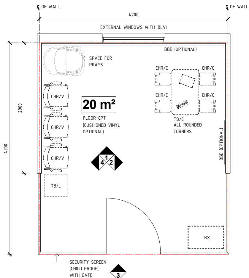
PLAN
