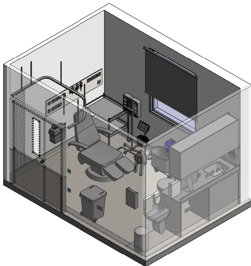
ISOMETRIC VIEW 01
