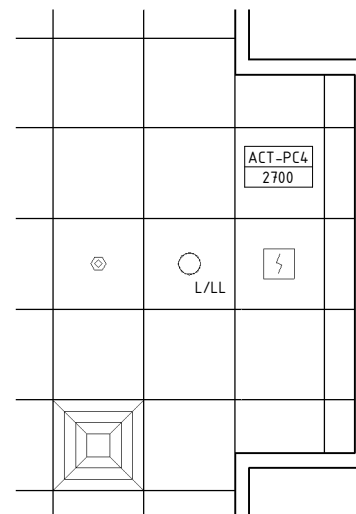
REFLECTED CEILING PLAN
