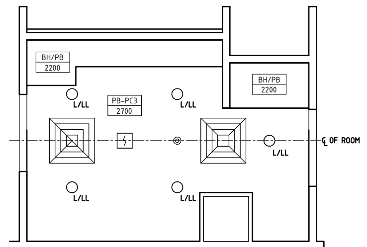
REFLECTED CEILING PLAN
