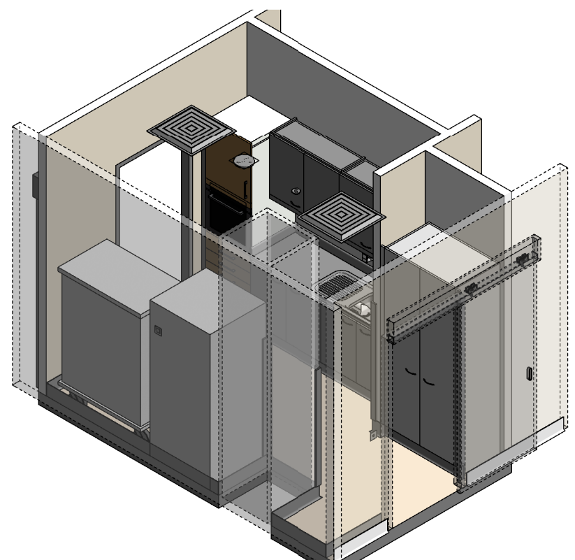
ISOMETRIC VIEW 02
