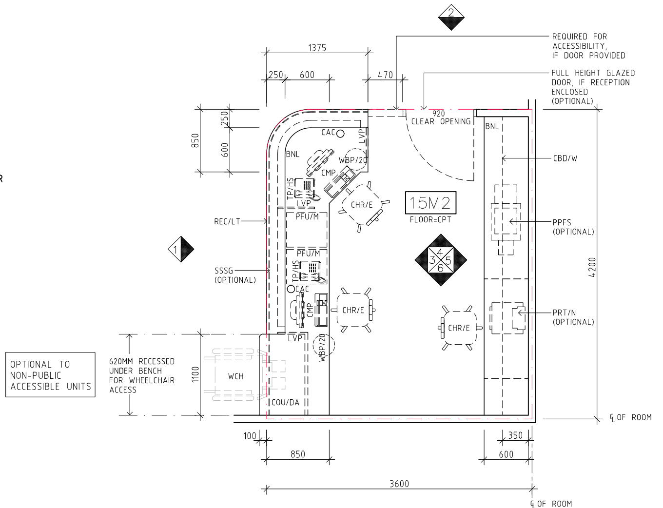
PLAN
