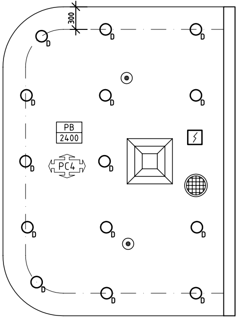
REFLECTED CEILING PLAN WITH BULKHEAD CEILING
