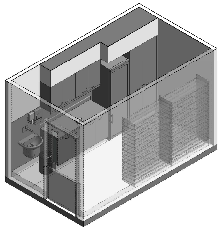
ISOMETRIC VIEW 2
