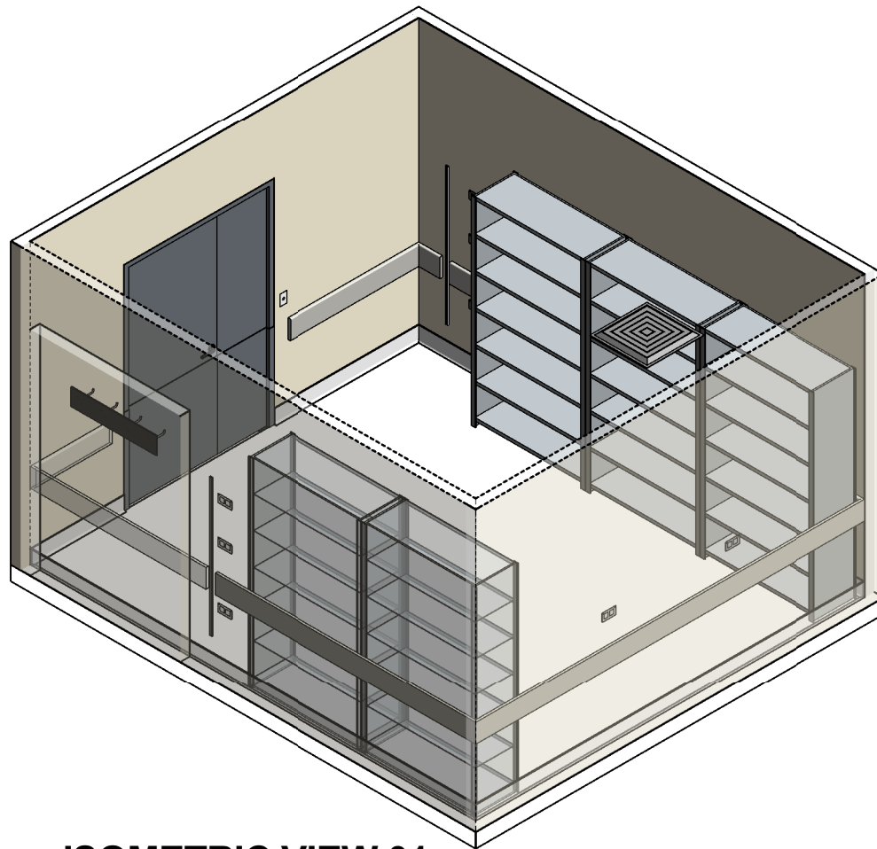
ISOMETRIC VIEW 01
