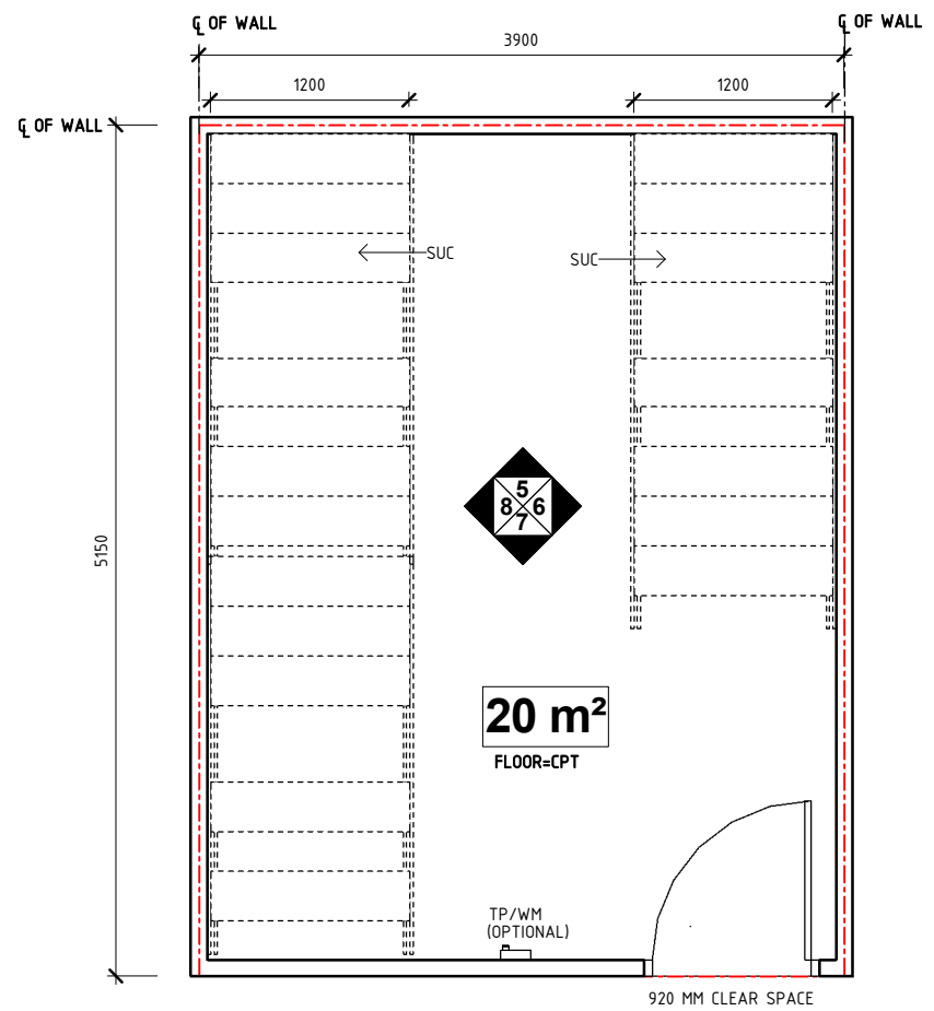
PLAN OPTION 2- COMPACTUS SHELVING PLAN
