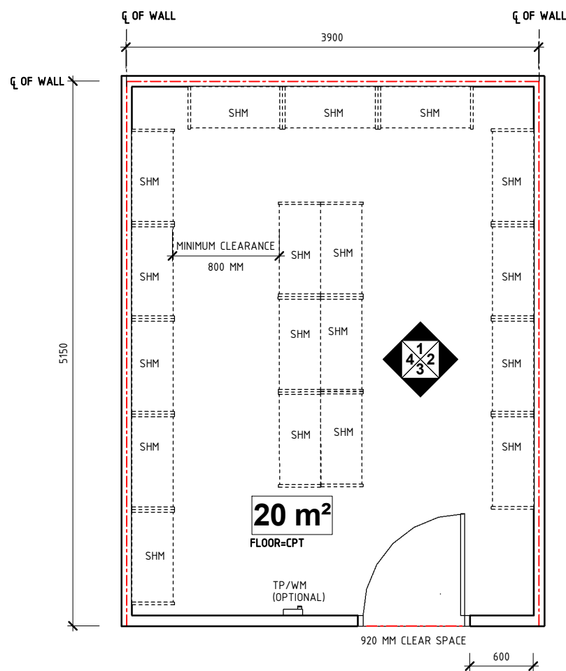
PLAN OPTION 1- STATIC SHELVING PLAN
