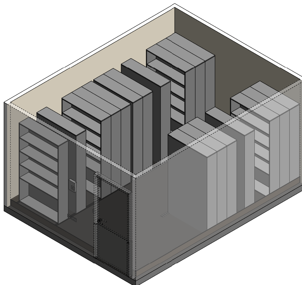
ISOMETRIC VIEW- (OPTION 2) OPTION 2- COMPACTUS SHELVING PLAN
