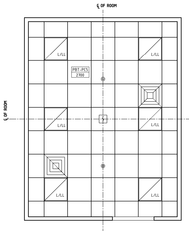
REFLECTED CEILING PLAN OPTION 1- STATIC SHELVING PLAN
