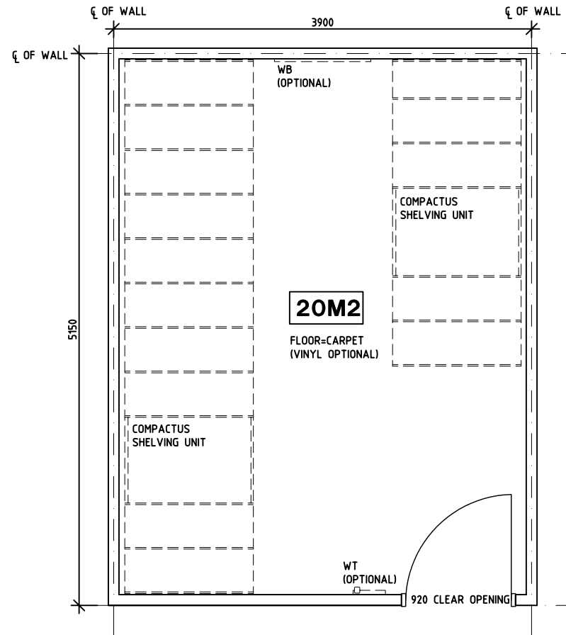
PLAN
