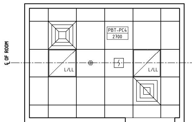
REFLECTED CEILING PLAN OPTION 1- STATIC SHELVING PLAN
