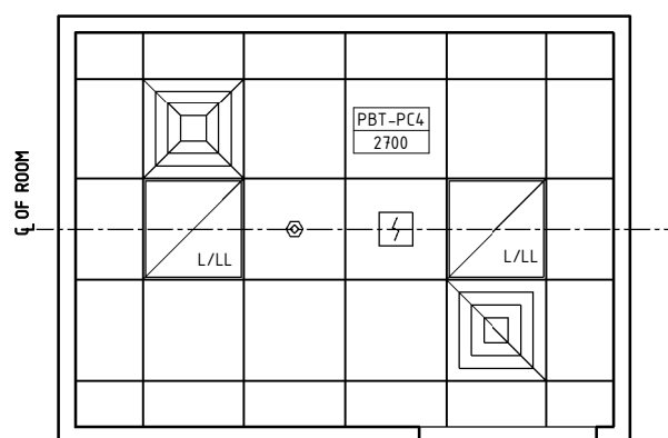
REFLECTED CEILING PLAN OPTION 2- COMPACTUS SHELVING PLAN
