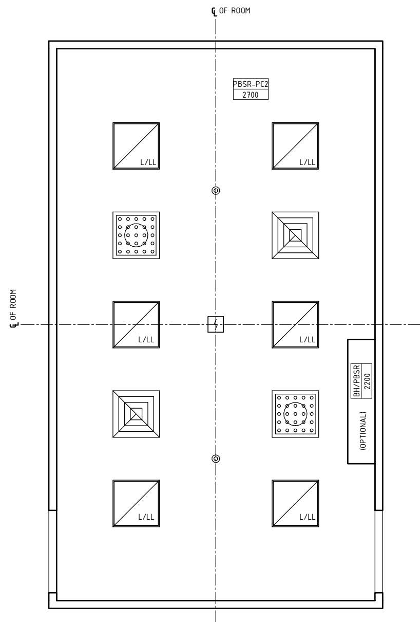
REFLECTED CEILING PLAN
