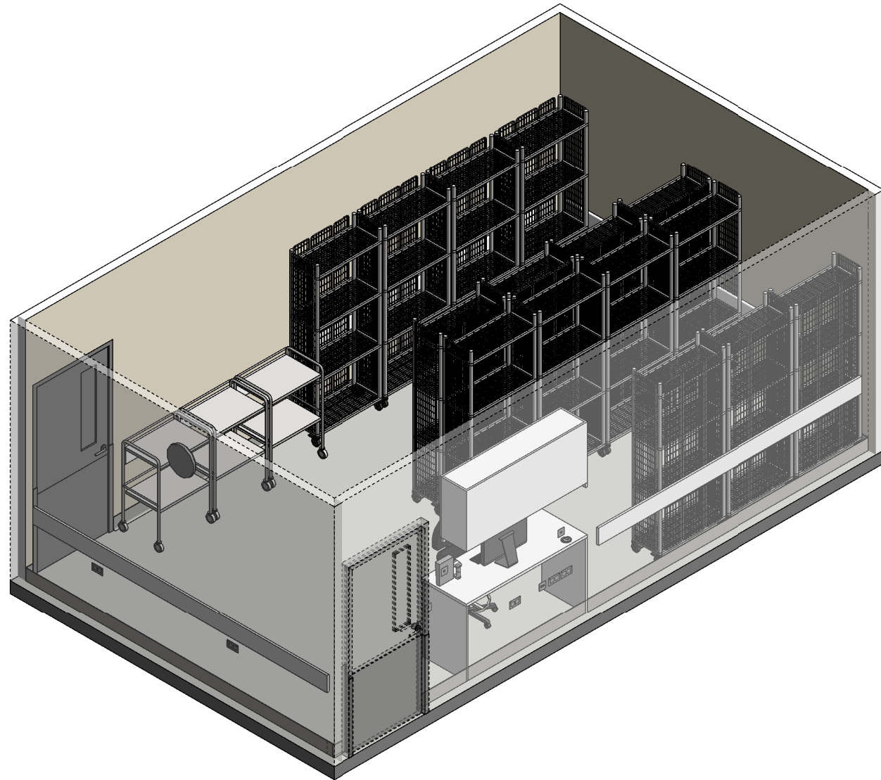
ISOMETRIC VIEW 01
