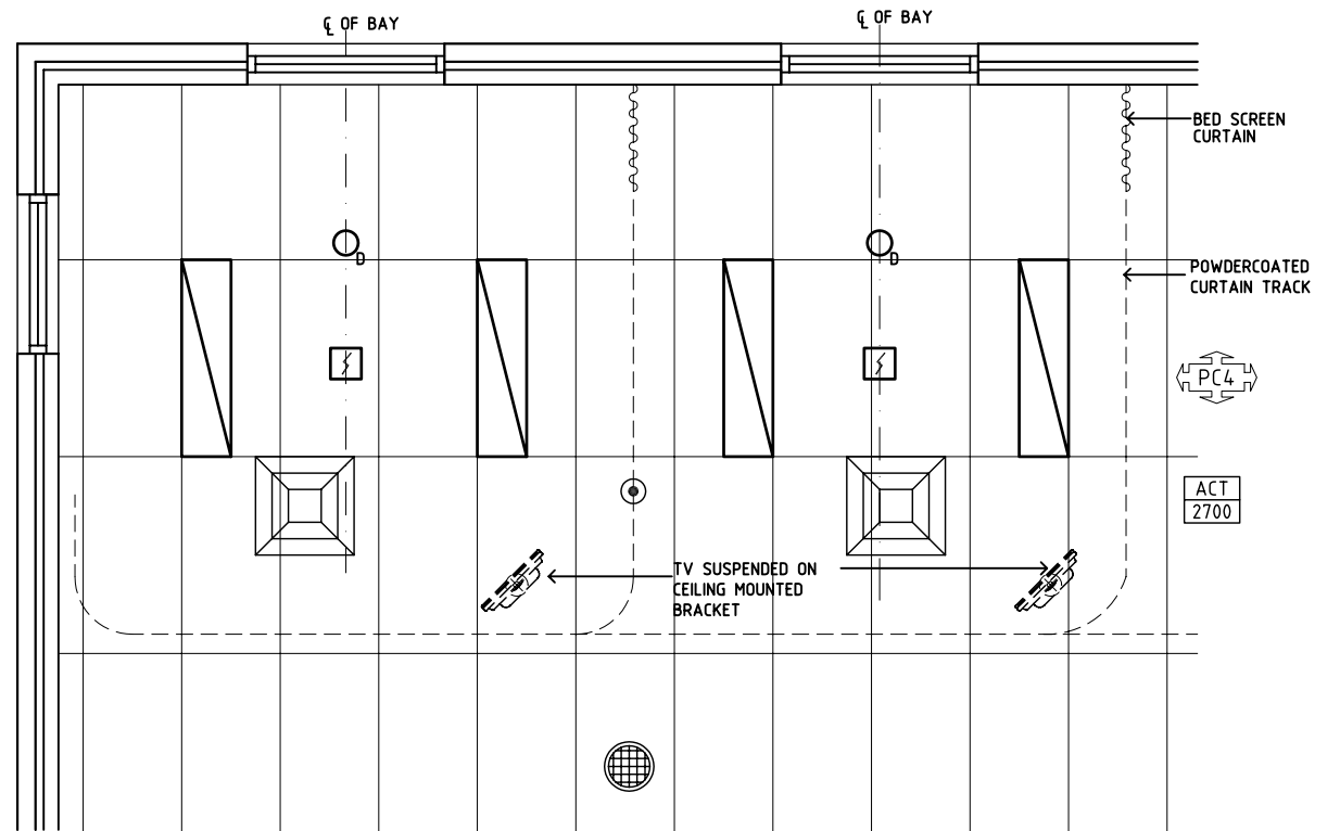
REFLECTED CEILING PLAN
