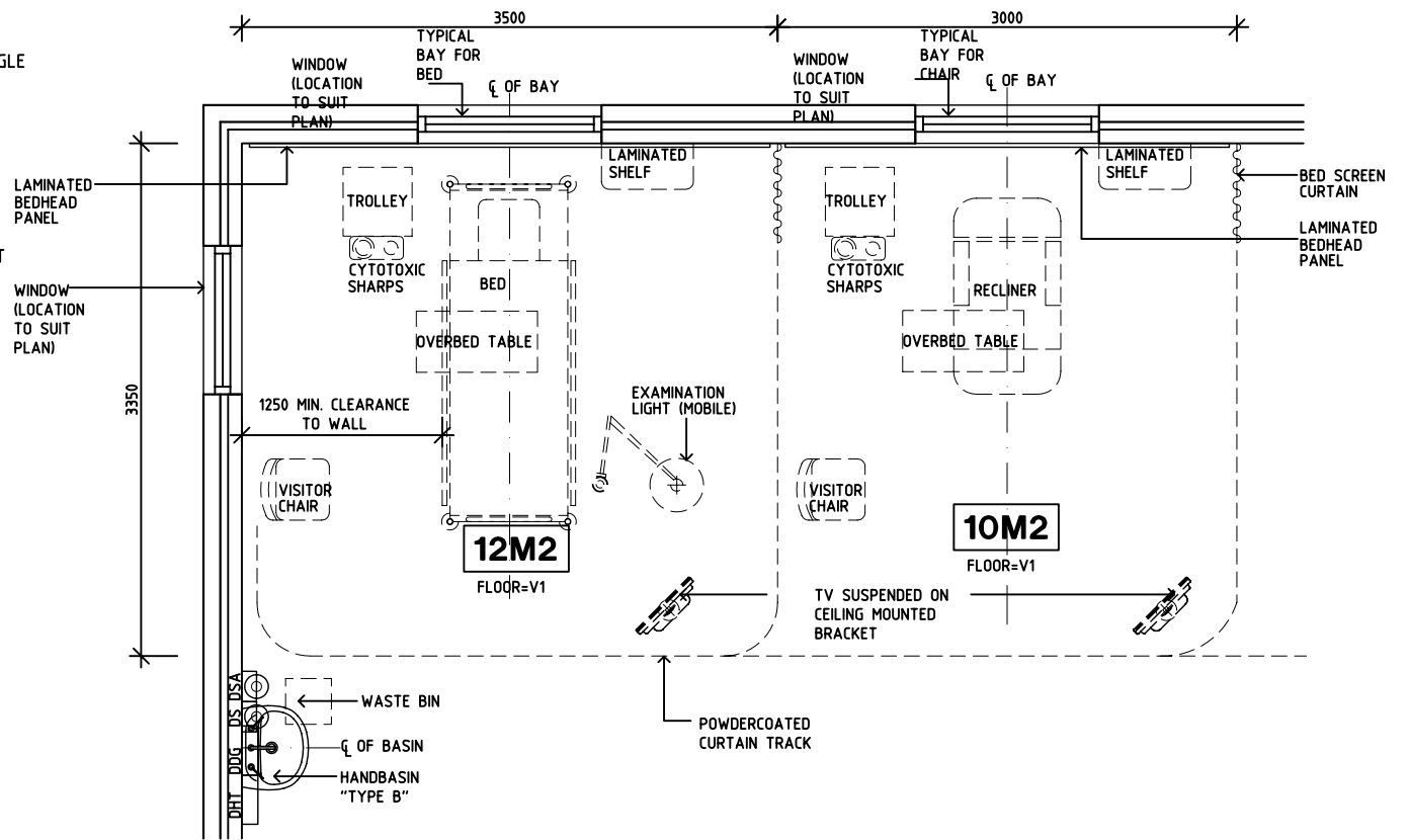
PLAN
