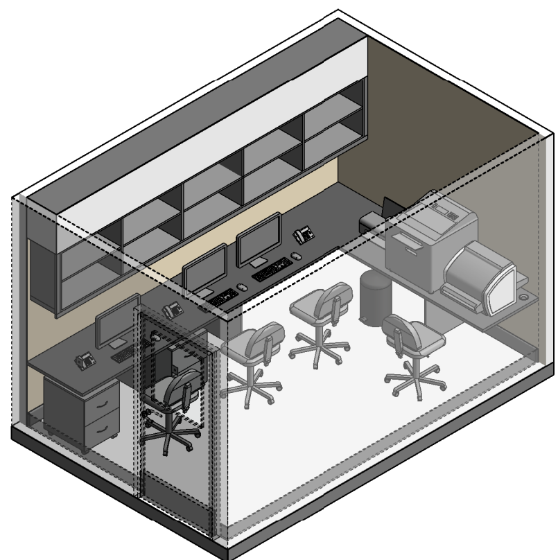
ISOMETRIC VIEW 2
