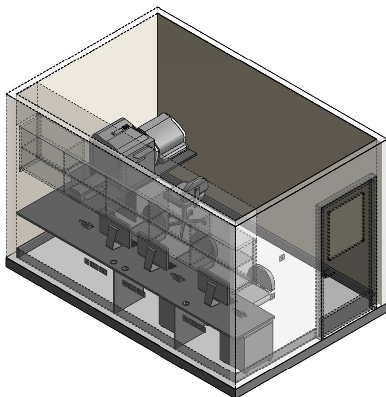
ISOMETRIC VIEW 1
