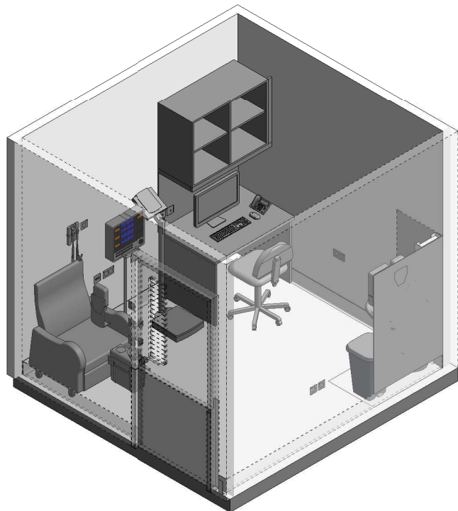
ISOMETRIC VIEW 01
