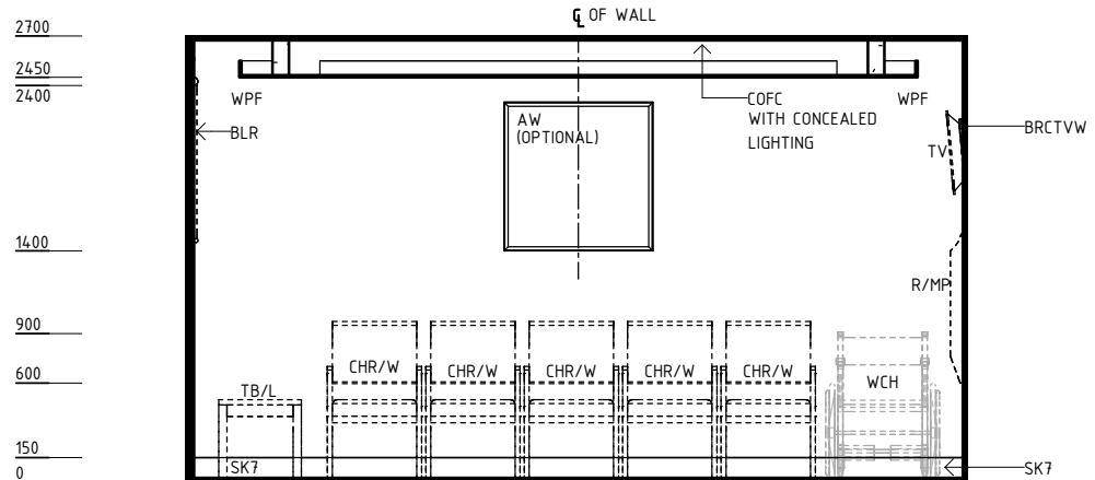
ELEVATION 2 ELEVATION 6 (MIRRORED)
