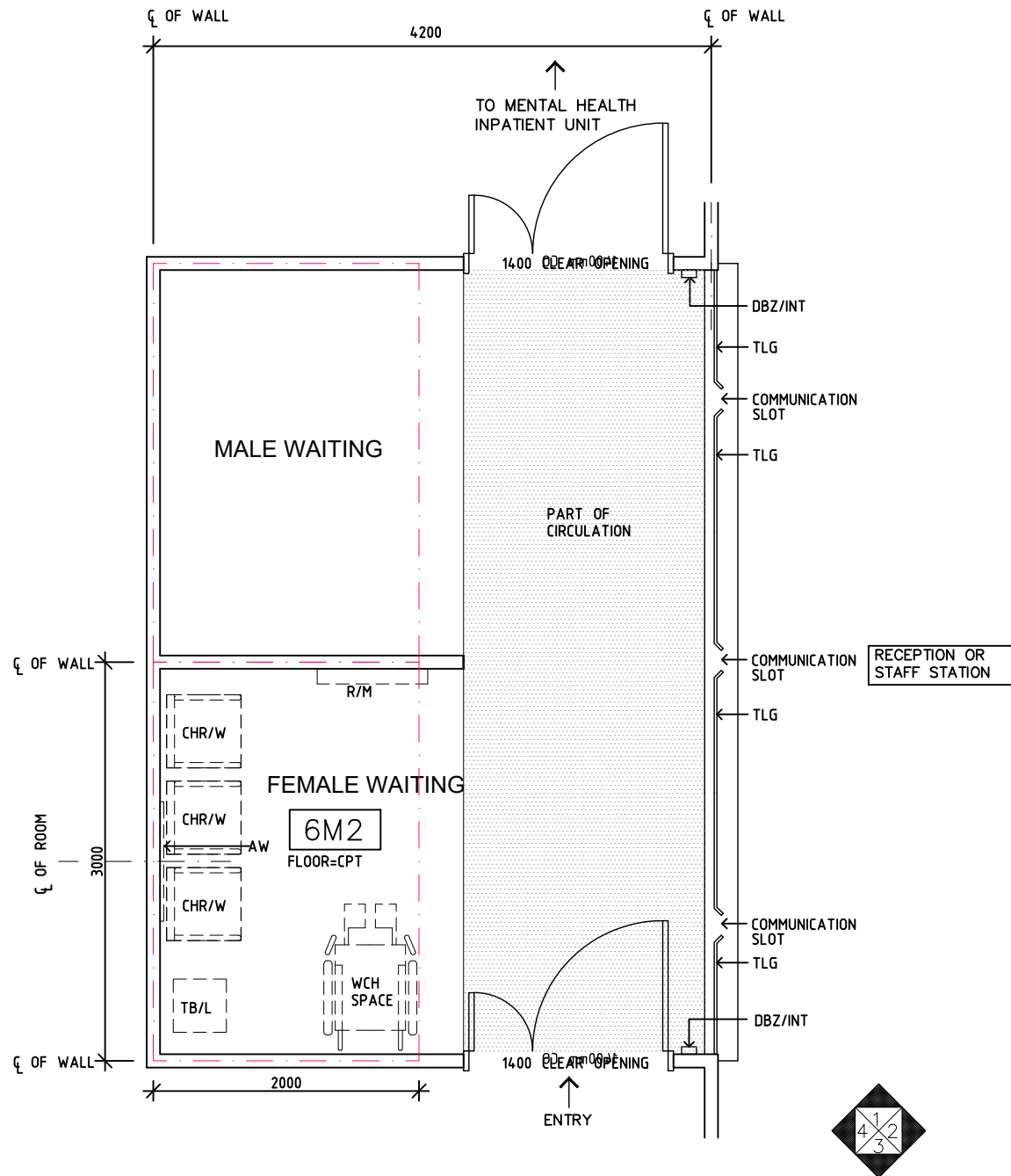
PLAN
