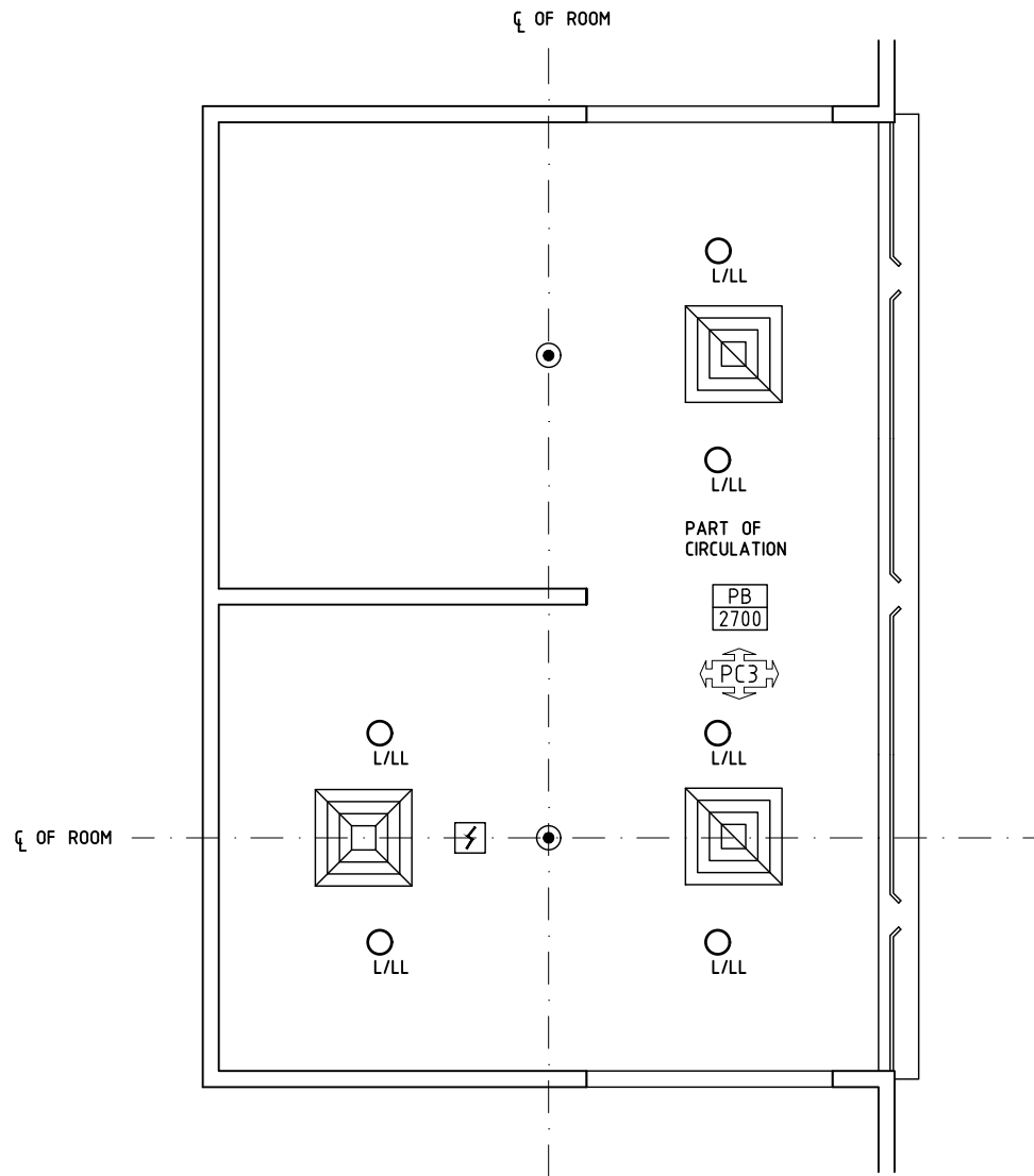
REFLECTED CEILING PLAN
