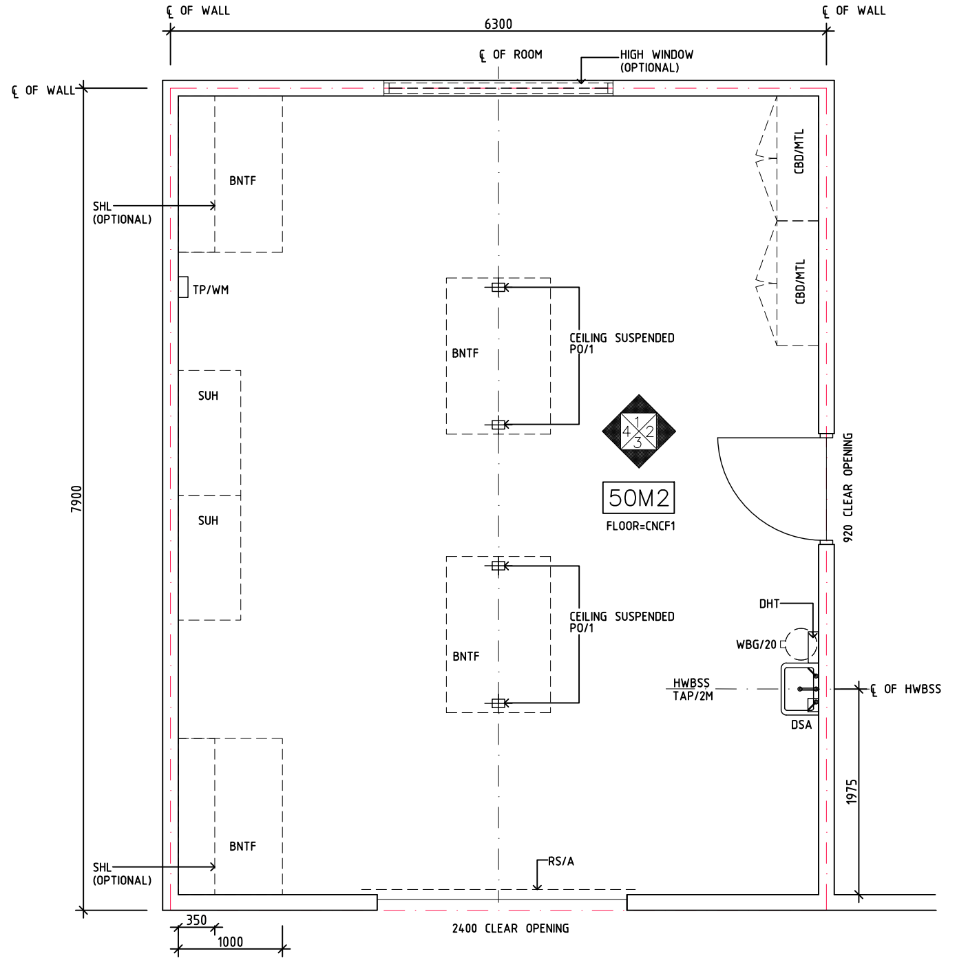
PLAN
