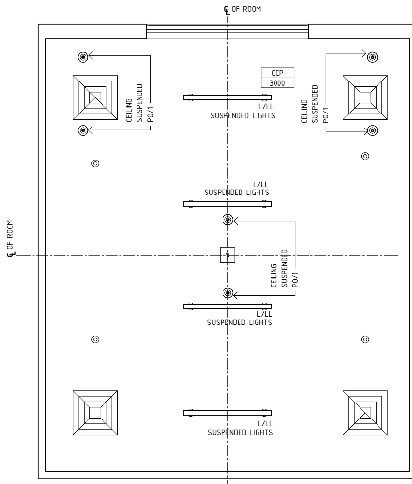
REFLECTED CEILING PLAN
