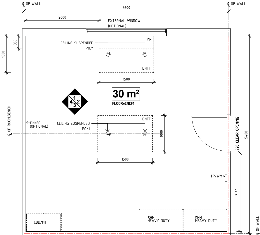
PLAN
