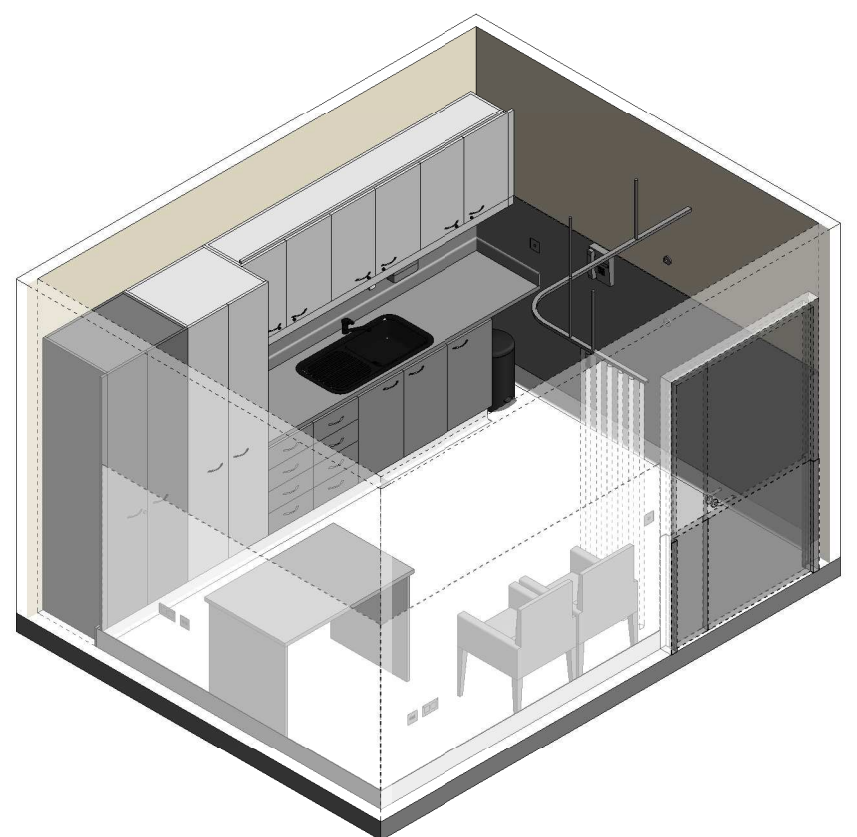
ISOMETRIC VIEW 02
